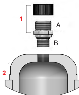
3K | 5K STANDARD GAS VALVE WITH CAPTURED O-RING SEAL
