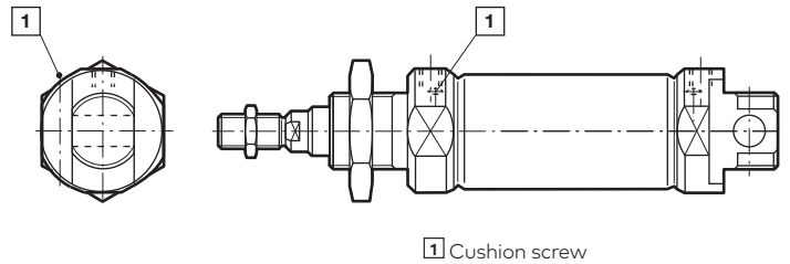
1 Cushion screw
